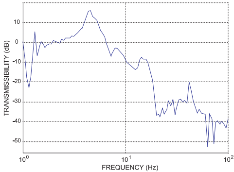
Vertical Transmissibility of Passive Isolation
